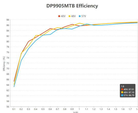
PoE Efficiency
