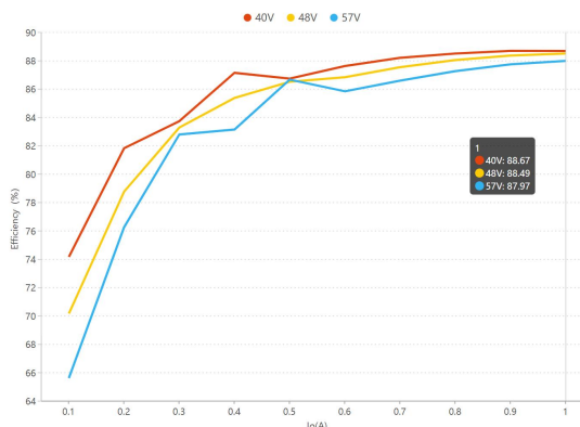
PoE Efficiency
