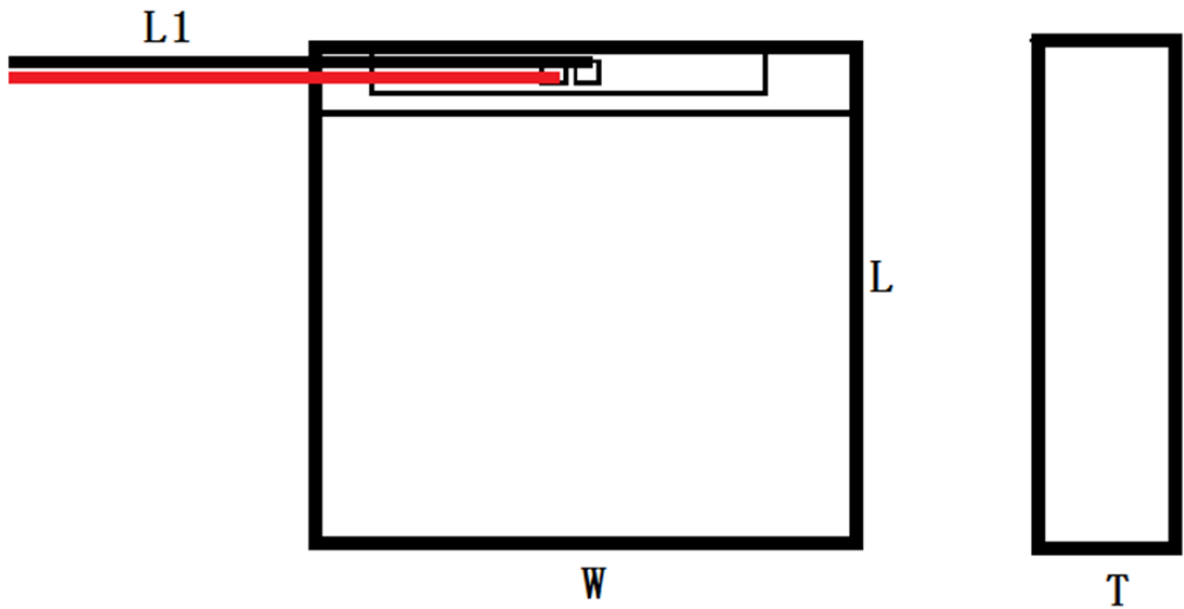
T=12.5mm(max), W=50.5mm(max), L=56.5mm(max) Battery
