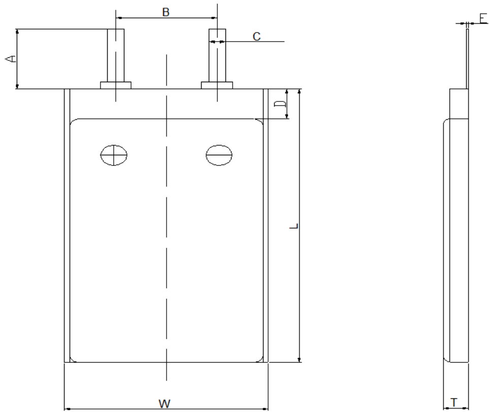
T=12.0mm(max), W=50.0mm(max), L=54.5mm(max) Cell
