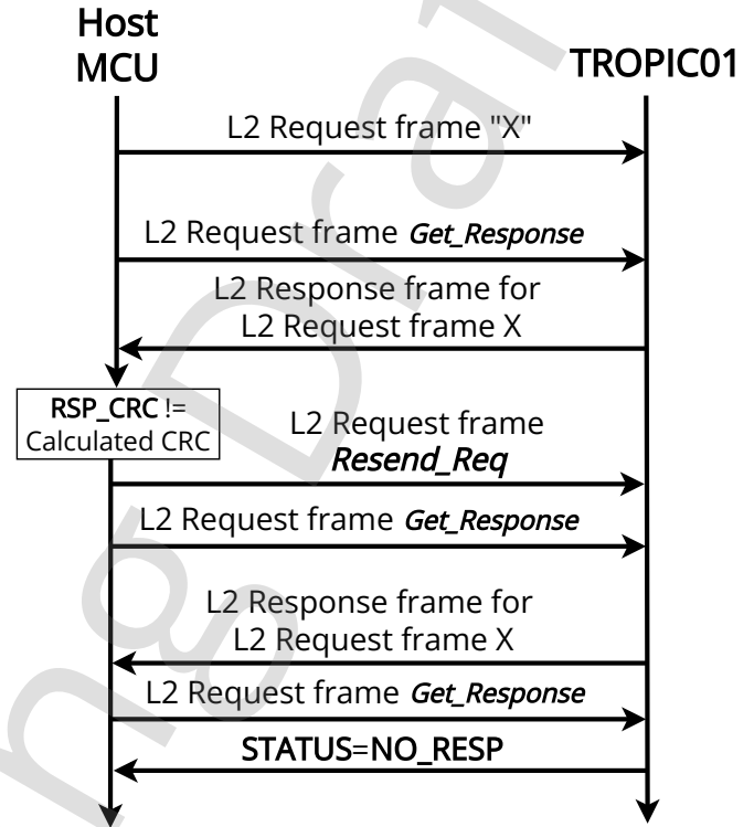
Figure 9: Resend_Req handling
