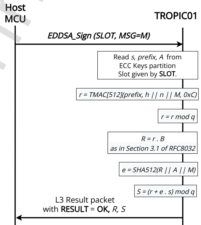
Figure 19: EdDSA Sign
